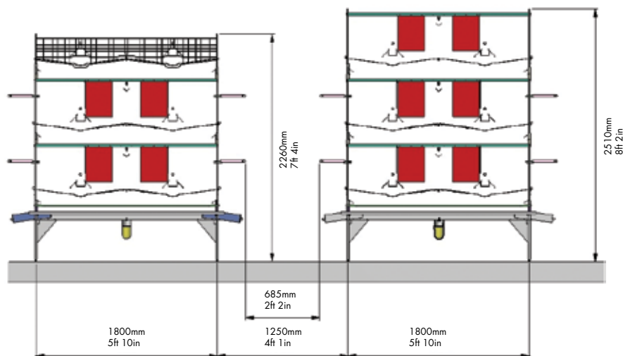
Example of two and three tier nest layout
