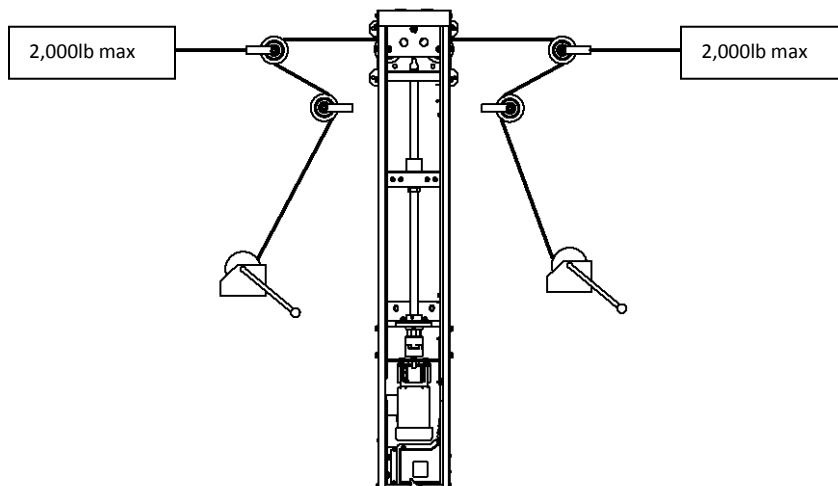
2:1 Ratio (Figure 11)
