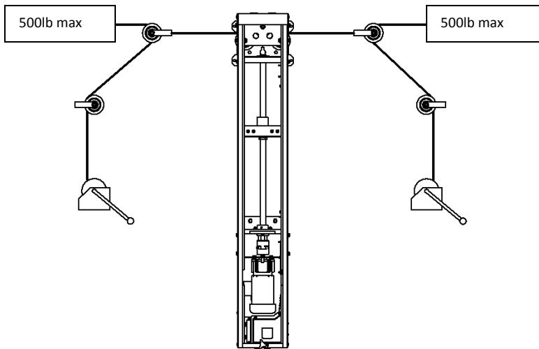
1:2 Ratio (Figure 10)
