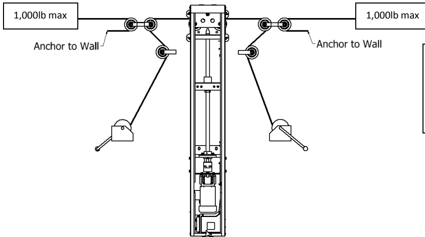
1:1 Ratio (Figure 9)
